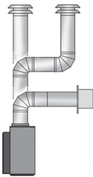
Standard venting configurations for: TC30, TC36, TC36 Arch, TC36 See-Thru, WS38, TC42, TC36 Outdoor and TC42 Outdoor
